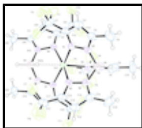
Fig. 1. The molecular structure of the title compound showing displacement ellipsoids drawn at the 35% probability level. H atoms are shown as spheres of arbitrary radius.
